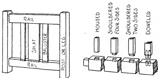
FIG. 396. JOINING SPLATS AND BALUSTERS TO RAILS.
